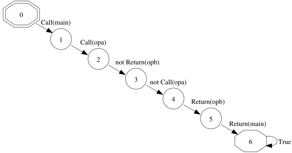
Figure 2.1: Automaton
