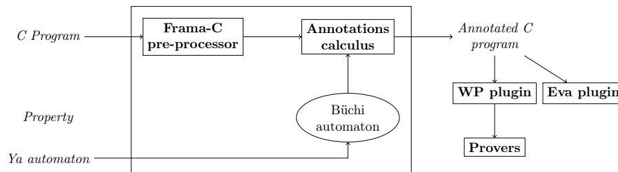
Figure 5.2: Plug-in Structure
